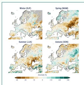
Seasonal soil moisture anomalies - Satellite
